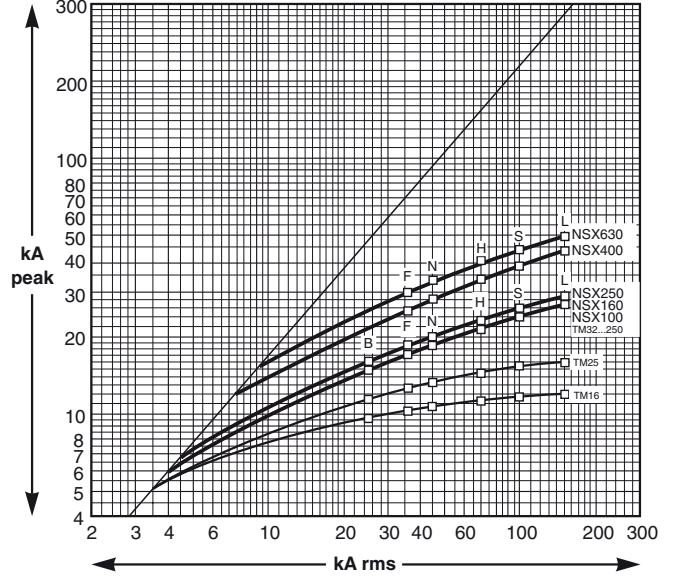
Compact NSX100 - 630
