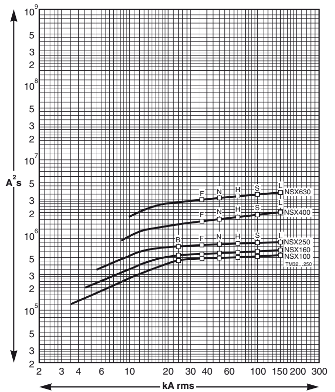
Compact NSX100 - 630
